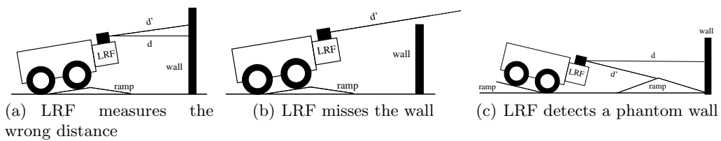
Fig. 7. Correct ( d ) and measured ( d' ) distances to walls due to ramps. (a): slightly incorrect measurement. (b) and (c): incorrect measurements that cause serious problems for the localization and the mapping.
