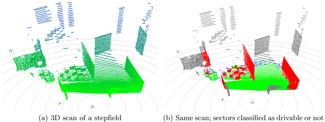
Fig. 9. Example of a 3D scan of the laser range finder.
