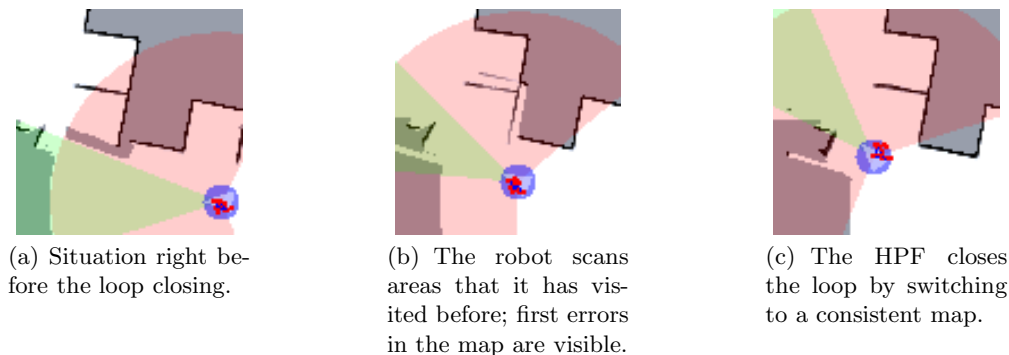
Fig. 5. Successful loop closing using a Hyper Particle Filter (HPF) with 30 particles.
