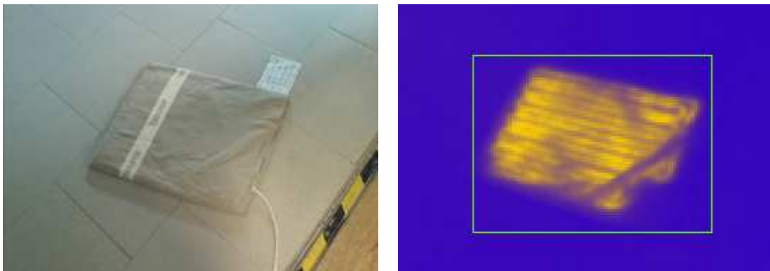
(a) A color image taken from one of the Sony FireWire cameras, showing a victim (electric blanket). (b) A thermal image created from the sensor data as shown in the GUI, showing the heat of the victim (inside the yellow bounding box).
