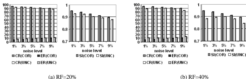
Figure 6: Quantitive evaluation for the segmentation results of uncorrected and corrected simulated images
