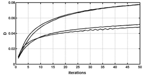
Figure 3: D_i curves for several tested images
