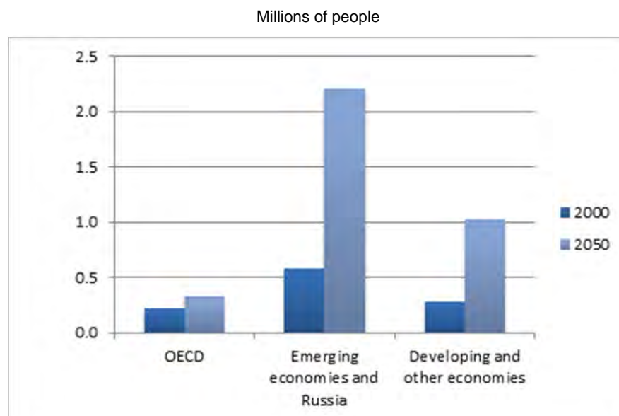
Figure 1.30. Premature deaths in urban areas from exposure to particulate matter (PM10) are projected to rise substantially in emerging economies by 2050
