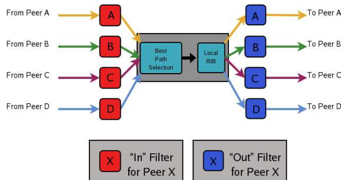
Figure 10.1: Announcement processing inside a “normal” BGP speaker
