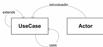
Figure 3 A meta-model of use-case diagrams
